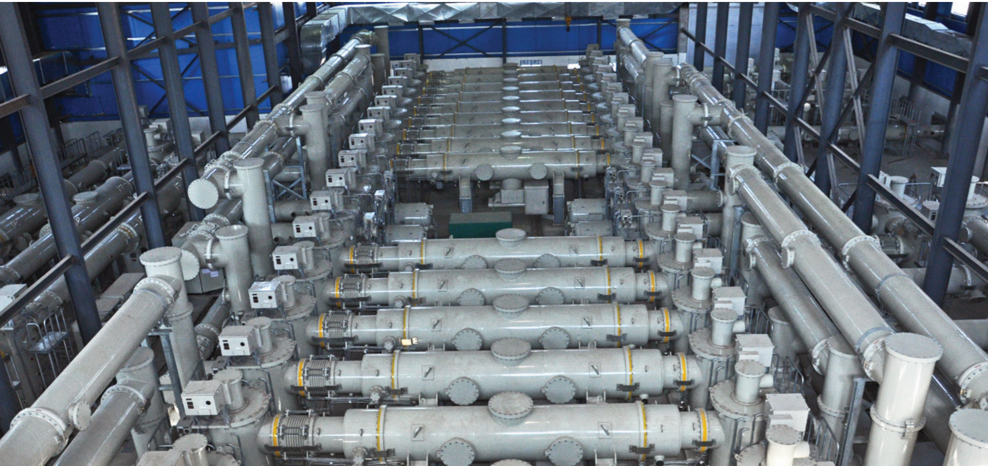
765 kV GIS at Pune
