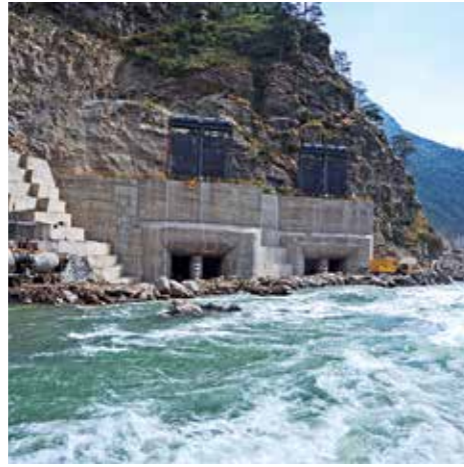
Intake structure at Punatsangchhu, Bhutan
