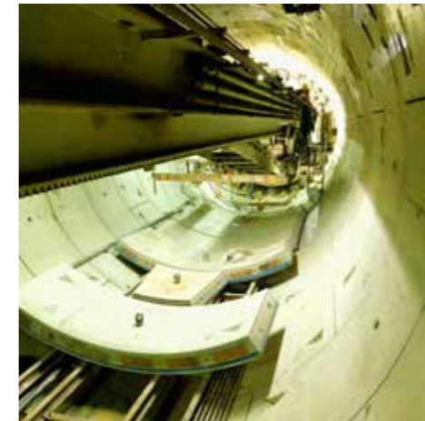
Ahmedabad Metro Tunnelling
